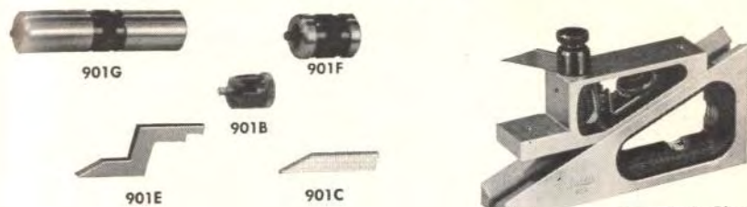
No. 901A Master Planer Gage with 901D attached
