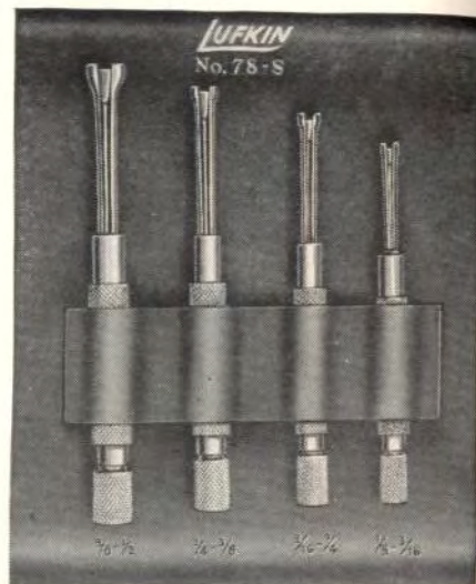
Complete Set No. 78S, Range 1/16 to 1/2-Inch
